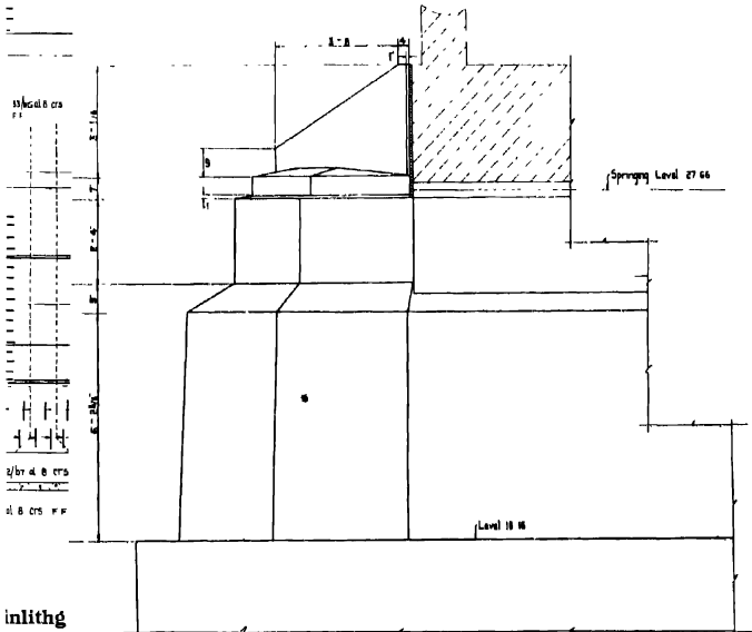
ENLARGED SIDE ELEVATION OF CUTWATER.
